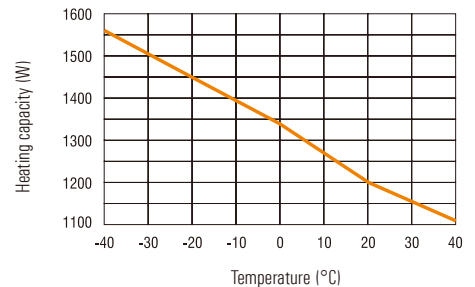
Heating capacity / Ambient temperature diagram CS 130
